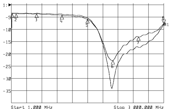
SR0901-2E: Port1 to Port2 and Port3
