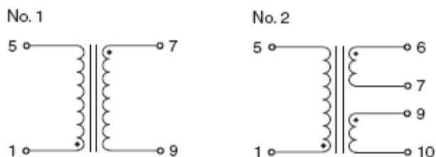
Circuit Diagram
