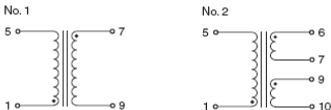
Circuit Diagram
