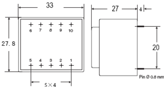
Dimension (mm)
