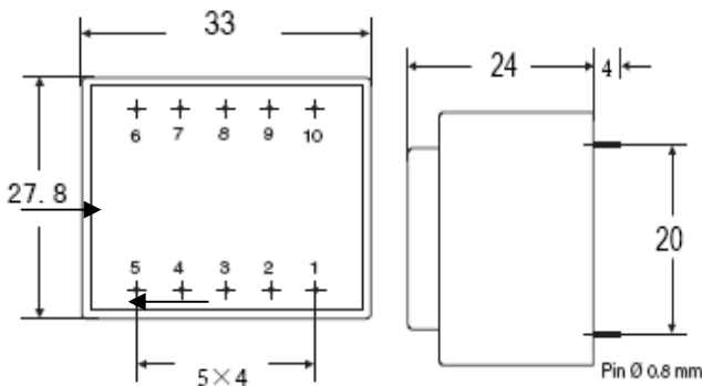
Dimension (mm)
