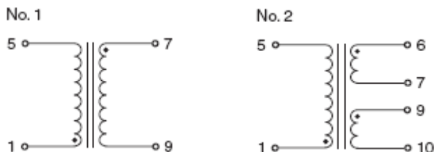
Circuit Diagram
